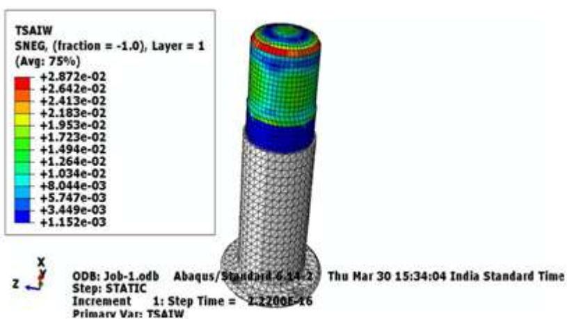
Figure 9 TSAIW Index (1.8mm)
