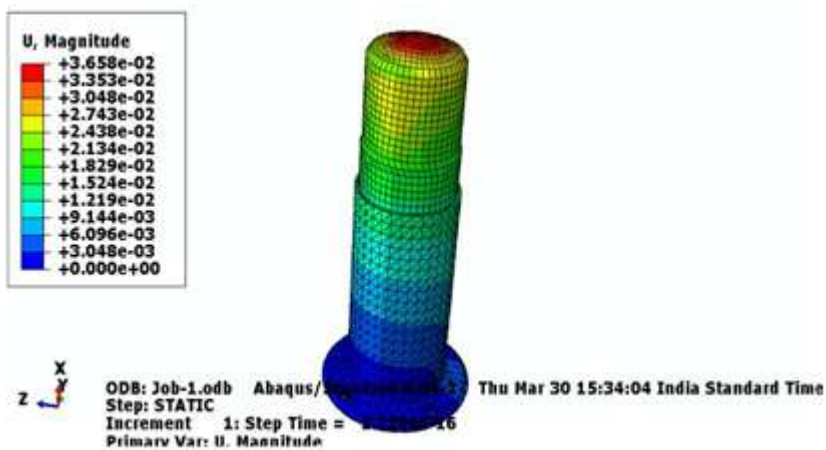
Figure 7 Displacement Contour (1.8mm)
