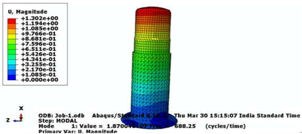
Figure 10 'Mode Shape 1', Frequency-60Hz (1mm)
