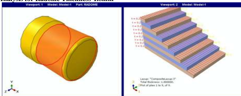
Figure 6 Layup Configuration (1.8mm)
