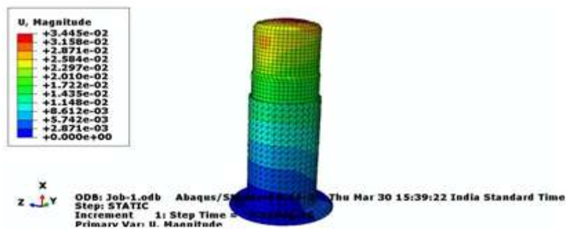
Figure 3 Displacement Contour (2mm)
